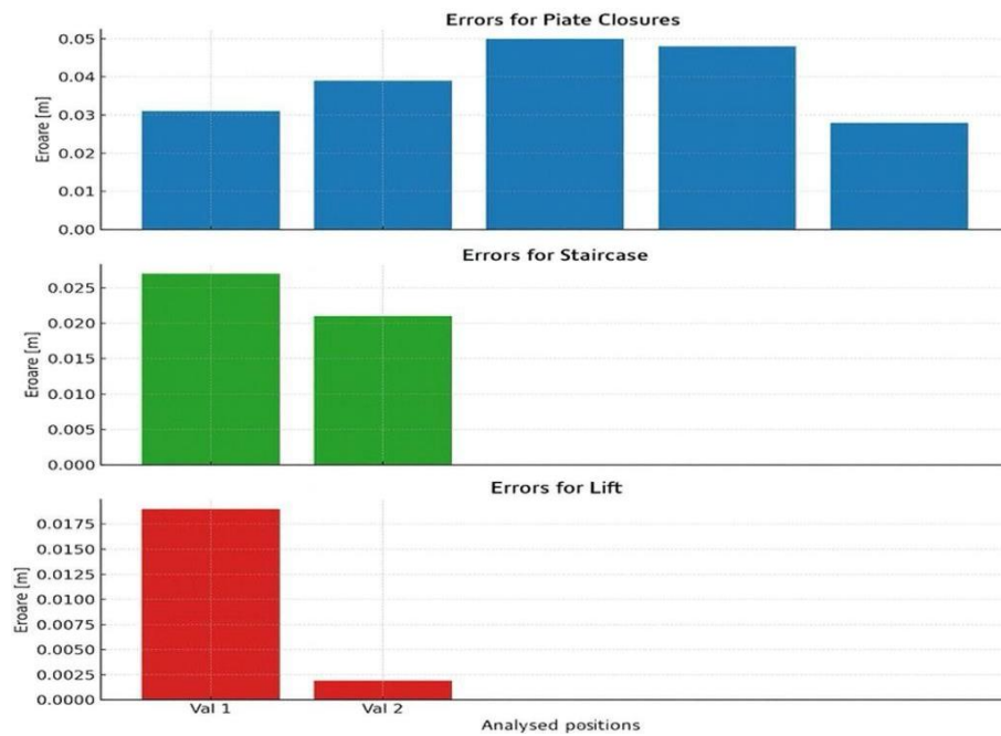
Fig. 9. Deviation graph.
