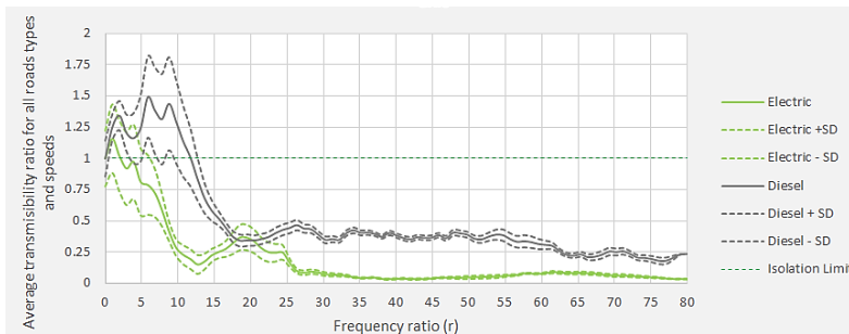
Fig. 8. Combined transmissibility [0–80] Hz for flat and ploughed land, speed 1 and speed 2, electric tractor model TE-0 and diesel tractor model TD80D.
