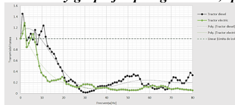
Fig. 6. Transmissibility graph, diesel tractor and electric tractor, frequency range [0–80] Hz
