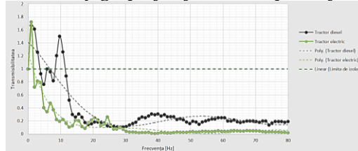
Fig. 4. Transmissibility graph, diesel tractor and electric tractor, frequency range [0–80] Hz
