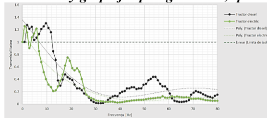
Fig. 5. Transmissibility graph, diesel tractor and electric tractor, frequency range [0–80] Hz
