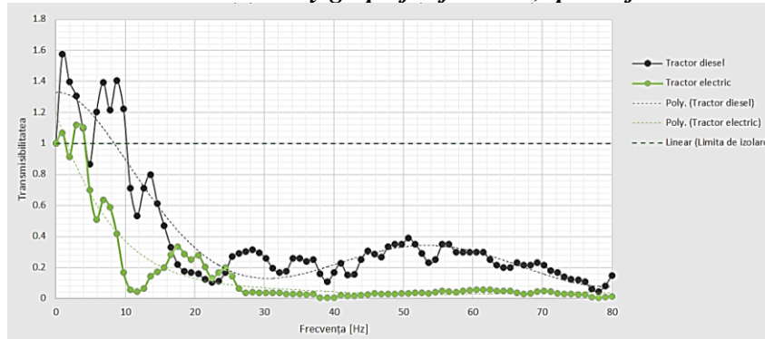
Case 1. Transmissibility graph for flat land, speed of 5 km/h
