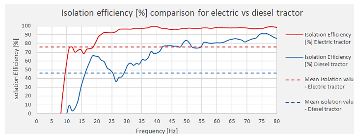
Fig. 10. Combined isolation efficiency [%] in the range [0–80] Hz for flat and ploughed land, speed 1 and speed 2, electric tractor model TE-0 and diesel tractor model TD80D.
