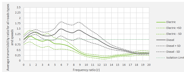
Fig. 7. Combined transmissibility [0–20] Hz for flat and ploughed land, speed 1 and speed 2, electric tractor model TE-0 and diesel tractor model TD80D.
