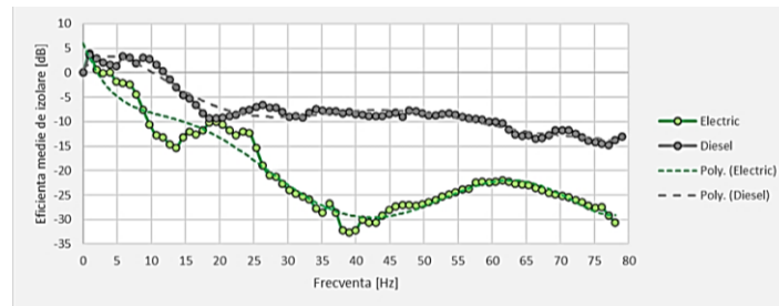
Fig. 9. Combined isolation efficiency [dB] in the range [0–80] Hz for flat and ploughed field, speed 1 and speed 2, electric tractor model TE-0 and diesel tractor model TD80D.
