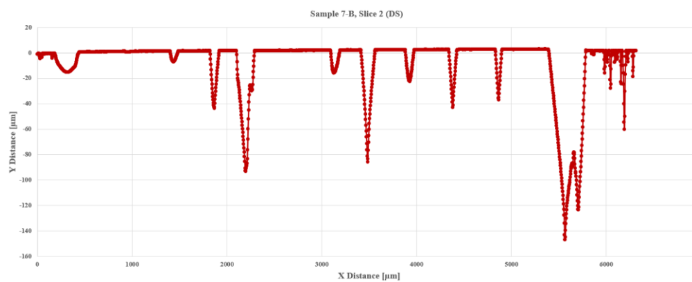
Variation of the slice 2 parameter for the dovetail -interface sample
