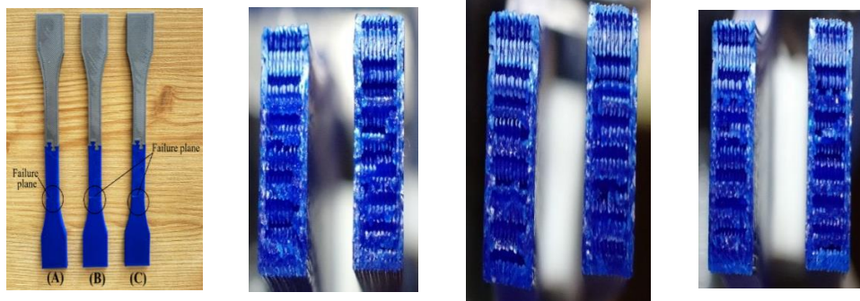
Fig. 3. Fracture regions of the 2T-interface samples: cross-sectional view of failure sample (A, B, C).
