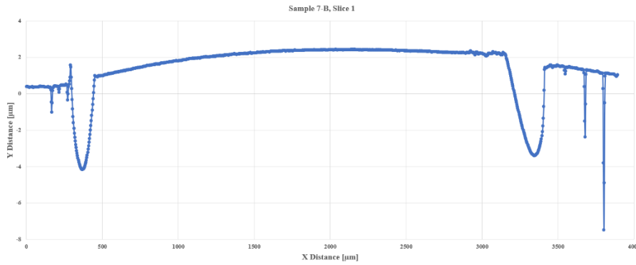
Variation of the slice 1 parameter for the T-interface sample
