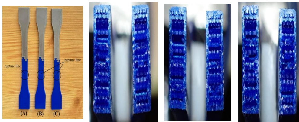
Fig. 5. Fracture regions of the double-dovetail -interface samples: cross-sectional view of failure sample.
