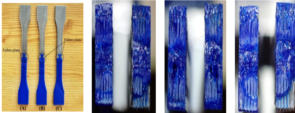
Fig. 2. Fracture regions of the T-interface samples: cross-sectional view of failure sample (A, B, C).
