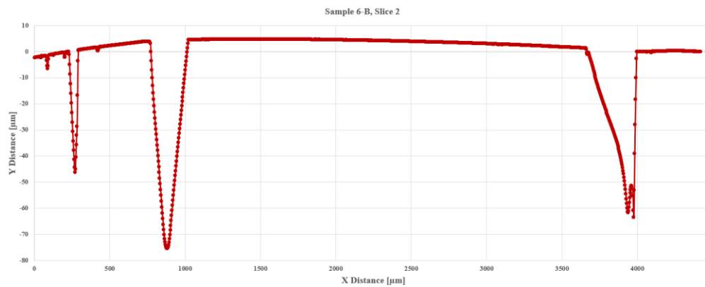
Variation of the slice 2 parameter for the 2T-interface sample
