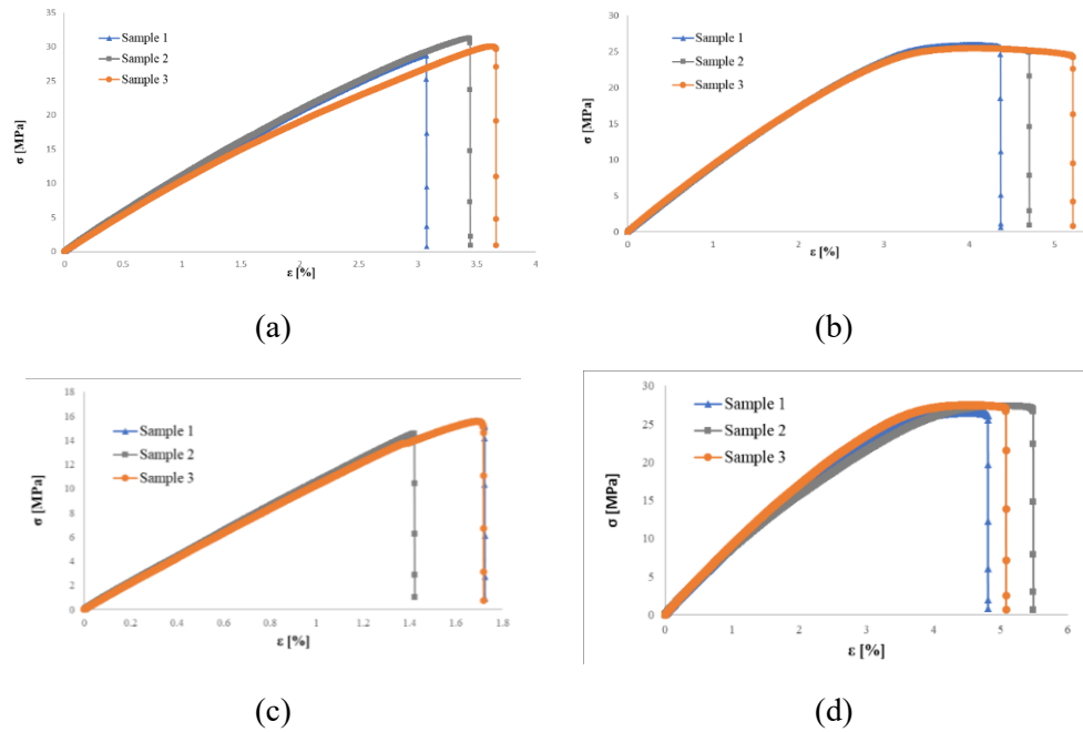
Fig. 1. Stress-strain behavior of bicomponent UltraFuse PLA-PLA/PHA 3D-printed samples: (a) T; (b) 2T; (c) dovetail; (d) double-dovetail
