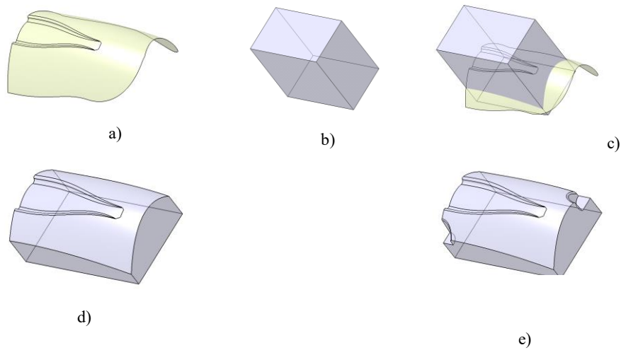
Fig.3. Modeling the mold ( method 1 )
