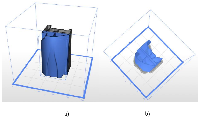
Fig.7. 3D printing simulation method 2 (hollow mold) a) Placement of parts to be printed in volum; b) 3D printing simulation,
