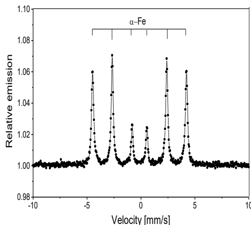
Fig. 3 CEMS spectrum of a corroded sample in a solution with 10^{-3} \text{HN}_3 concentration with NCBSA inhibitor (● data; — fit; --- \alpha -Fe).
