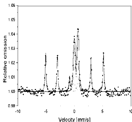
Fig. 4 CEMS spectrum of a corroded sample in a 1 HCl solution (● data; — fit; -o- \alpha -Fe; - \Delta - doublet 1; - \nabla - doublet 2)
