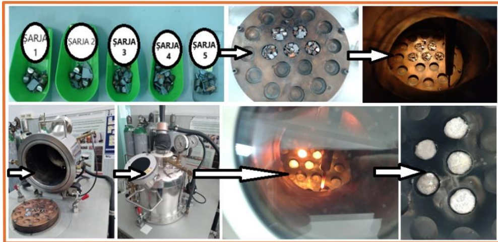
Fig. 1. Stages of the obtainment of experimental alloys by vacuum arc remelting using the VAR ABJ 900 system.
