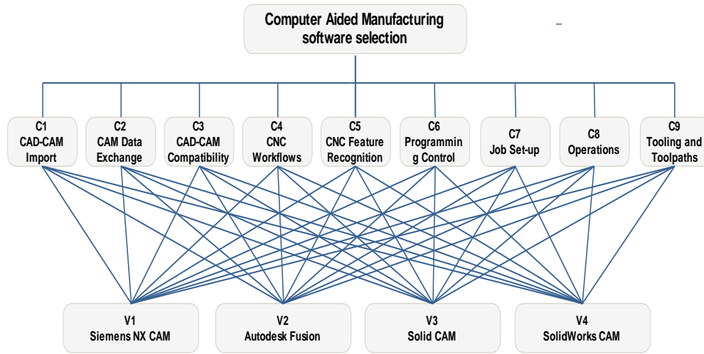
Fig. 1. Hierarchical structure.
