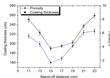
Fig. 28. Variation of coating thickness (μm) and porosity (%) as a function of spray distance [104].
