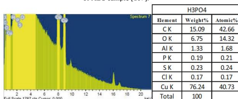
Fig. 35. EDX for different copper coatings in \text{H}_3\text{PO}_4 bath: a) EDS spectra; b) elemental analysis of ABS sample [107].
