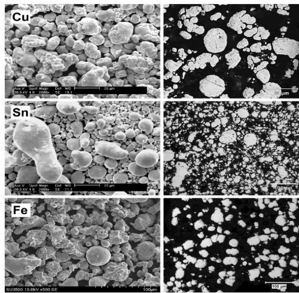
Fig. 6. SEM images (left) and cross-sectional optical micrographs (right) of raw material powders, [58, 59].
