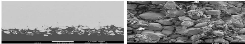
Fig. 19. The characteristics of the intermediate penetrated zone at the Cu/PEEK interface: a) penetration of copper powders over an area of about 100 μm thickness; b) weakly deformed zone due to PEEK deformation [87].
