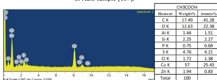
Fig. 37. EDX for different copper coatings in \text{CH}_3\text{COOH} bath: a) EDS spectra; b) elemental analysis of ABS sample [107].
