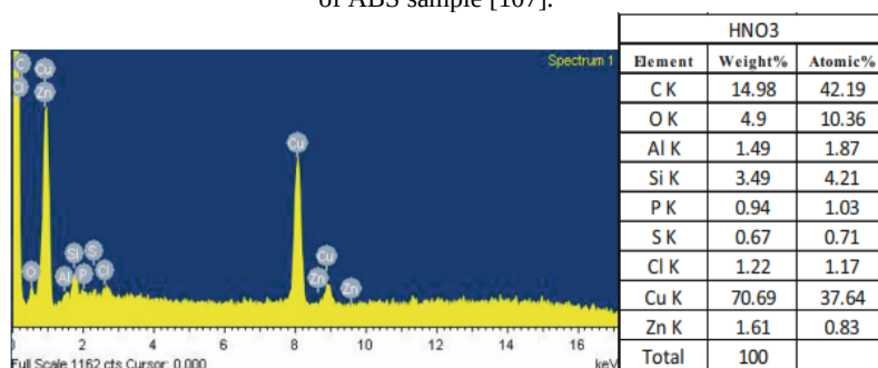
Fig. 36. EDX for different copper coatings in \text{HNO}_3 bath: a) EDS spectra; b) elemental analysis of ABS sample [107].
