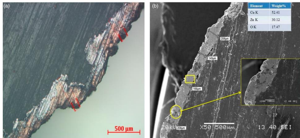
Fig. 25. SEM images of copper thermal spray coating: a) Optical micrograph showing three distinct layers of ABS, Zn and Cu; b) SEM images showing cross-sectional view of Cu-coated ABS, together with EDS analysis [101].
