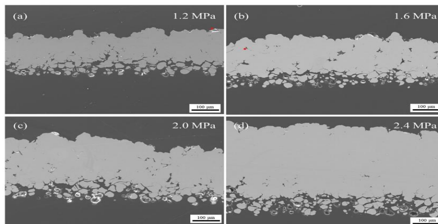
Fig. 15. Cross-sectional morphology of Cu coating on PEEK substrate at different propellant gas pressures: a) 1.2 MPa; b) 1.6 MPa; c) 2.0 MPa; d) 2.4 MPa, [82]
