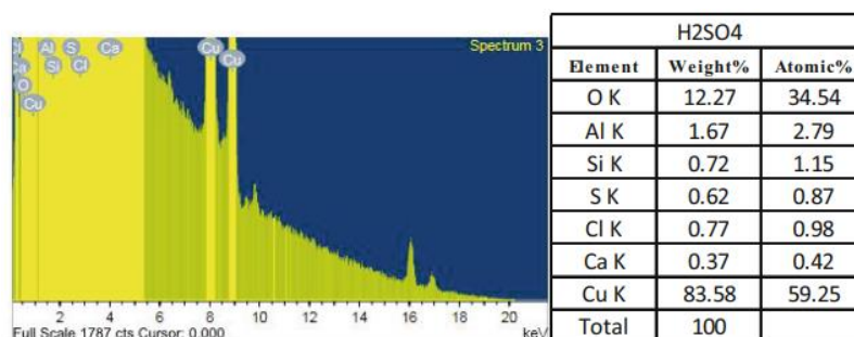
Fig. 34. EDX for different copper coatings in \text{H}_2\text{SO}_4 bath: a) EDS spectra; b) Elemental analysis of ABS sample [107].
