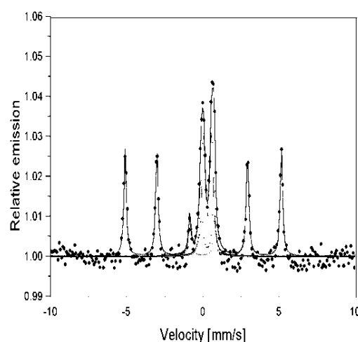
Fig. 6. CEMS spectrum of a corroded sample in a 1 HCl solution
