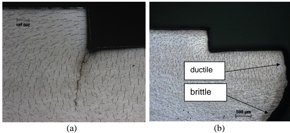
Fig. 4.2. Crack initiation (a) and rupture (b) in mechanical fatigue tests on samples with bearing pad-like defects.
