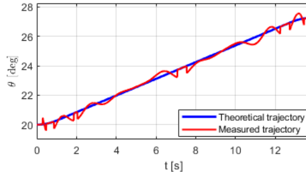
Fig. 13 The ProHep-LCT needle insertion robot comparative. time history diagram for the \theta coordinate of the end-effector.
