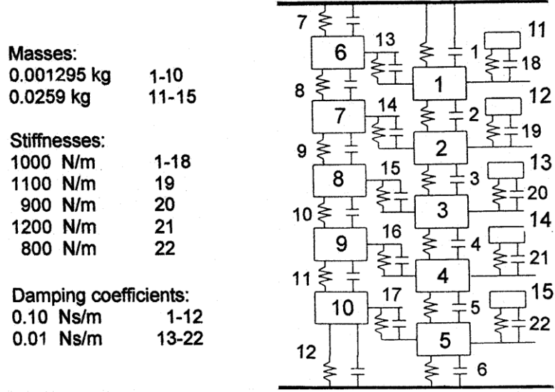
Fig. 1. 15 DOF system.
