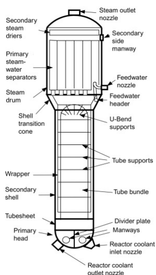
Fig. 3. CANDU Steam Generator.
