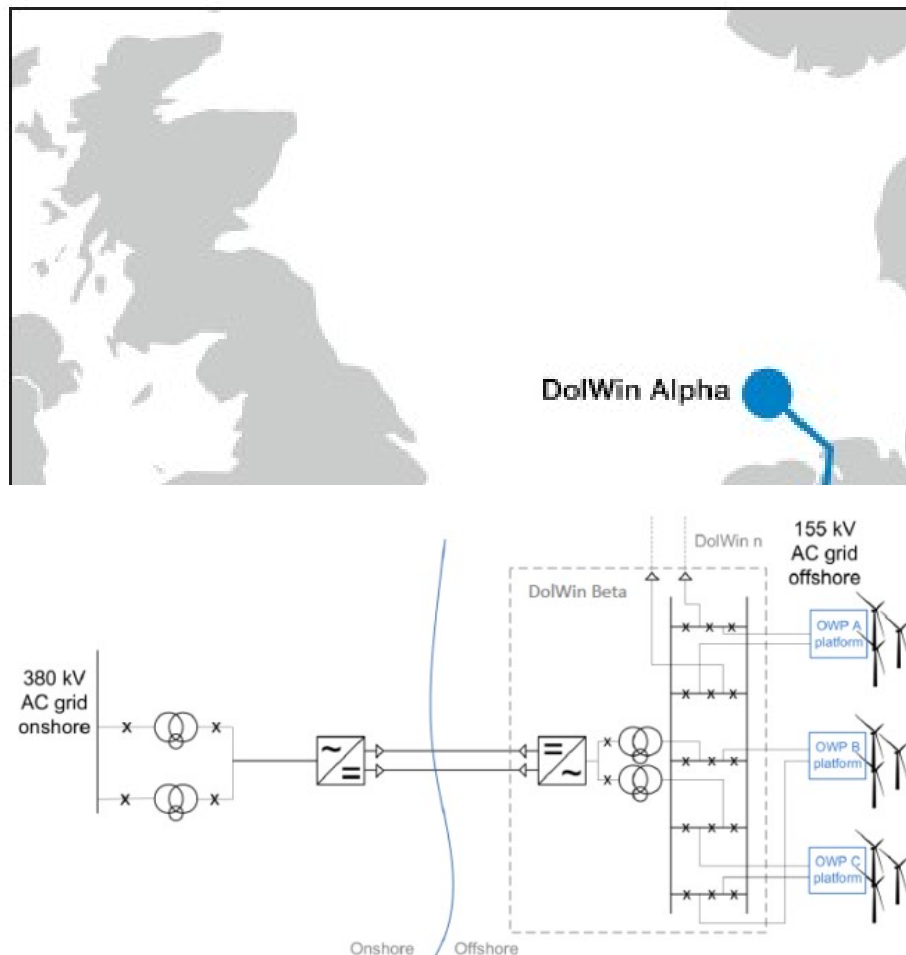
Fig. 16. HVDC connection "offshore" - "onshore" (Germany) [16].
