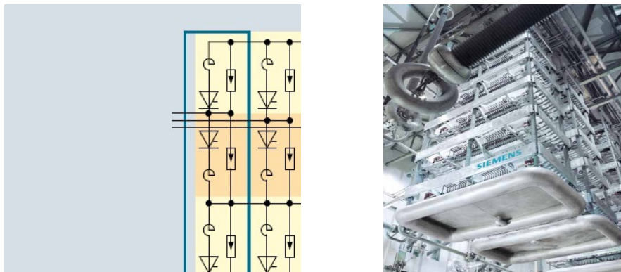
Fig. 5. 12 pulses controlled rectifier (AC-DC conversion) scheme and picture [7].
