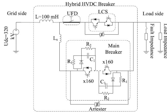
Fig. 7. Hybrid switching breaker schematics [10].
