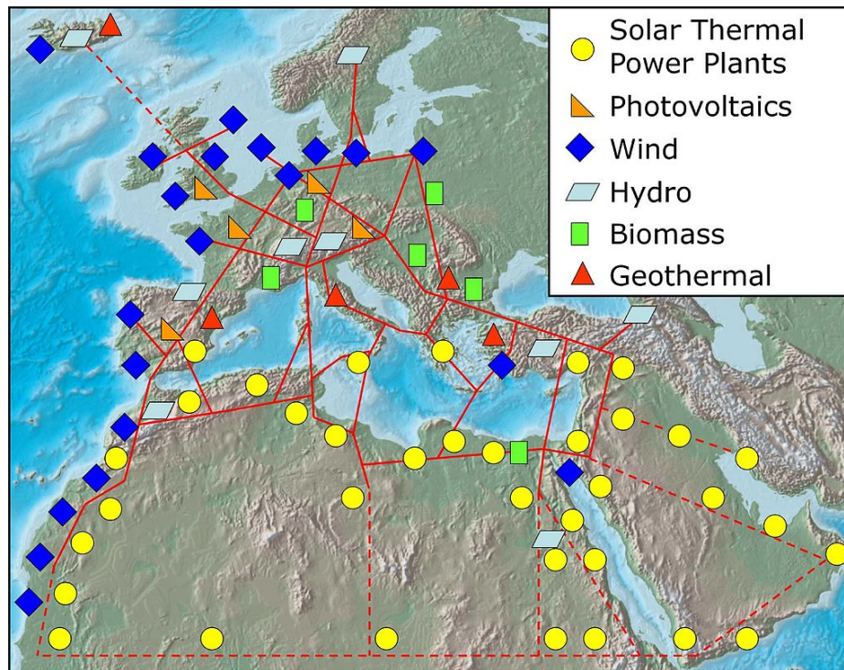
Fig. 17. The future proposed European super grid.
