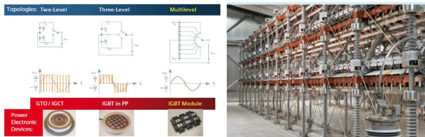
Fig. 9. a) Topologies and switching devices used in the construction of voltage inverters [6]; b) a voltage inverter picture.
