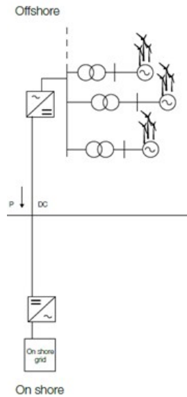
Fig. 4. HVDC for offshore wind power stations [8].
