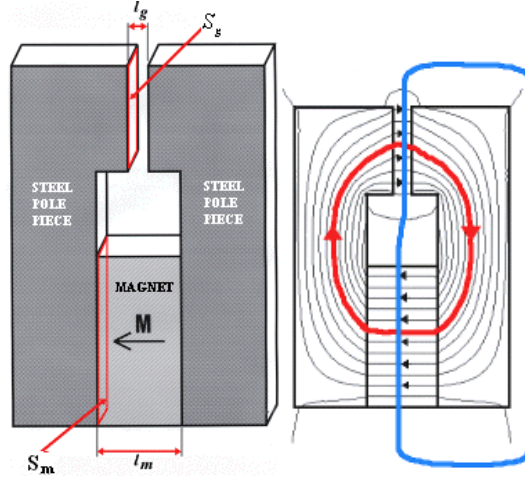
Fig. 7. Magnetic circuit indicating the circuit of applying Ampere law (red) and Gauss theorem (blue).
