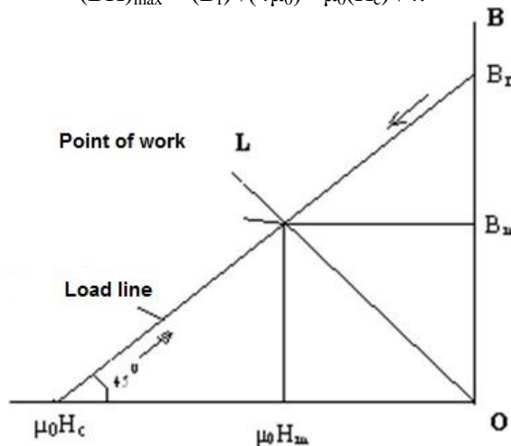
Fig. 9. The demagnetization curve of an ideal magnet.
