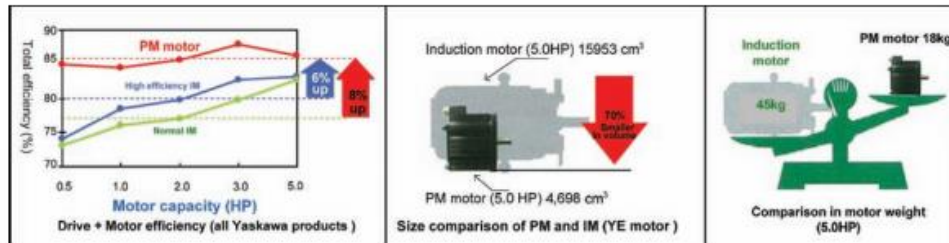
3. Some advantages of a PM motor over an induction motor (IM). Reproduced with permission.[33]
