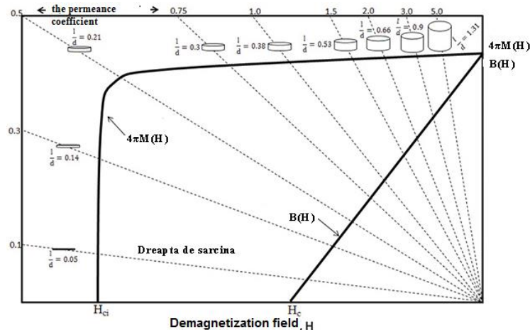
Fig. 4. Permeance coefficients for a PM with different dimensional ratios, corresponding load lines in B (H) and 4\pi M(H) representation.
