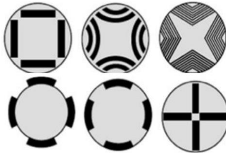
Fig. 10. Layout modes of PM in the rotor of a synchronous motor, shown here in a section perpendicular to the machine axis.
