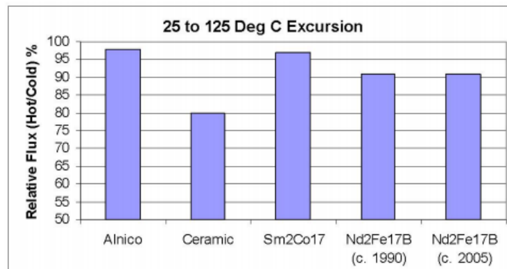
Fig. 6. Reversible losses at 125°C for various materials used to produce PM.
