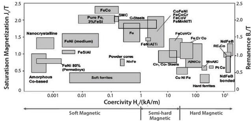
Fig. 1. Ordinary permanent magnets represented in the plane (remanence, coercivity).
