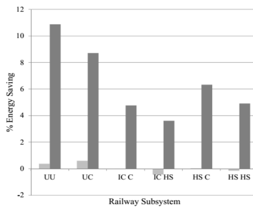
Fig. 12. Energy saving when replacing the induction motors with PM ones in different railway systems.
