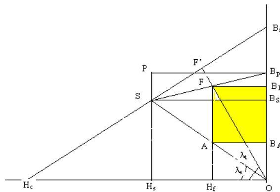
Fig. 8. PM in the representation of (B, H), defining the main circuit elements.
