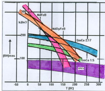
Fig. 5. The specific magnetic energy variation at PM from NdFeB, Alnico and SmCo families.
