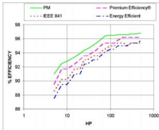
Fig. 11. Comparison of the efficiency of different types of electric motors.
